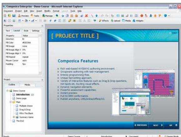
Authoring environment
